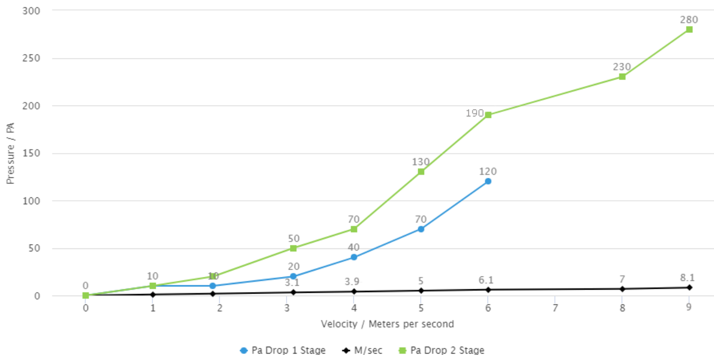
Single Stage & Two Stage Pressure Drop Data
